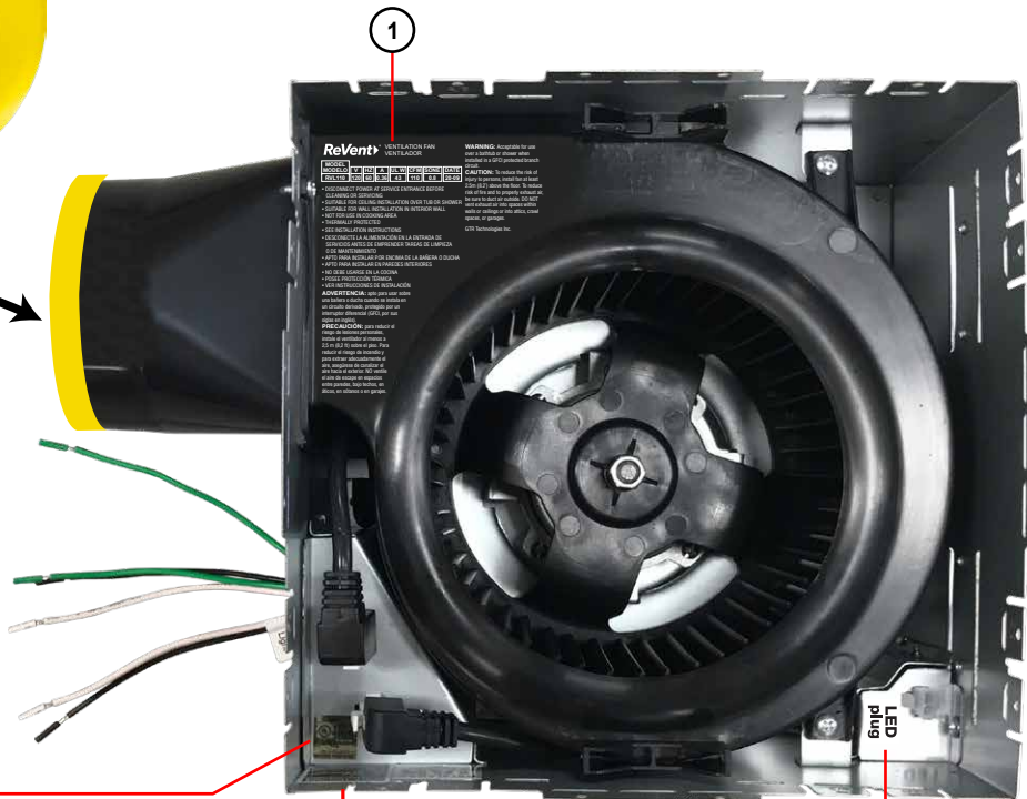
RVP-829-YL-01 4" damper cover
